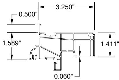
② MAIN FRAME HEAD/JAMB/SILL EQUAL LEG UPVC / VINYL-FLANGE
