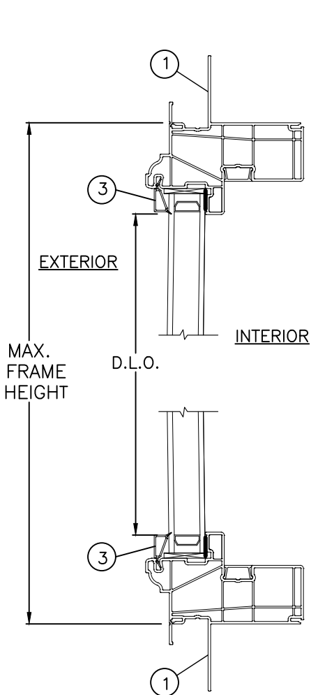
A 8 VERTICAL SECTION FRAME HD/SILL
