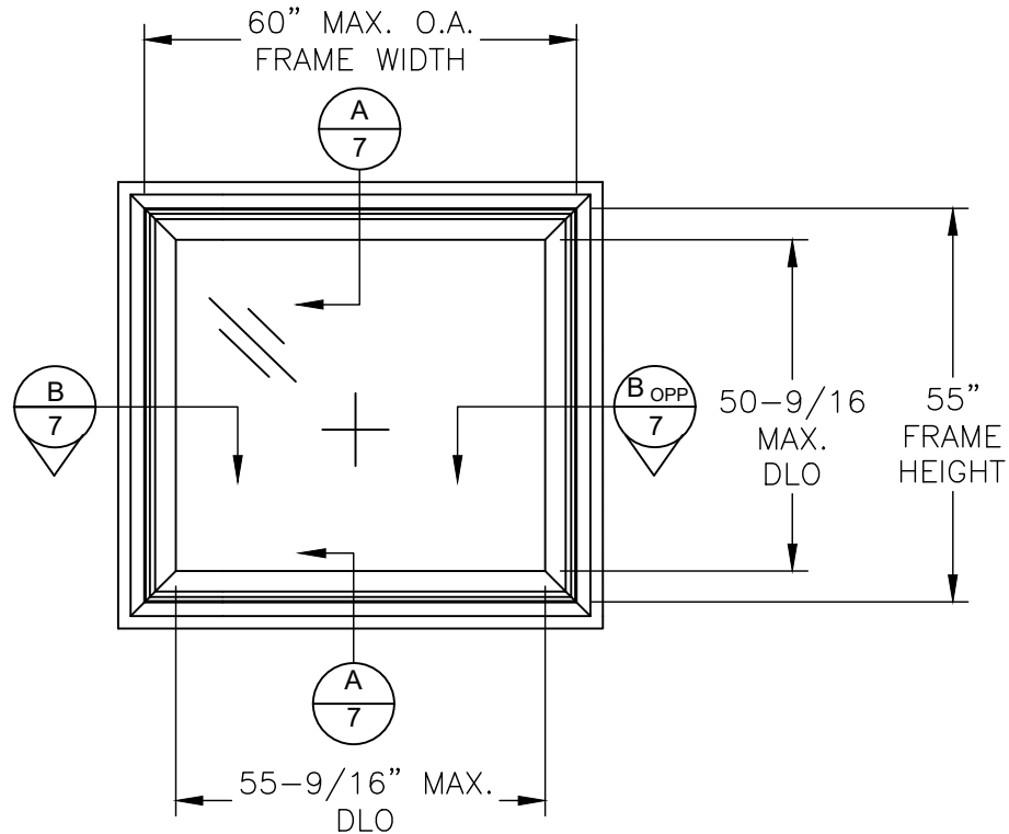
ELEVATION LAYOUT PICTURE WINDOW
