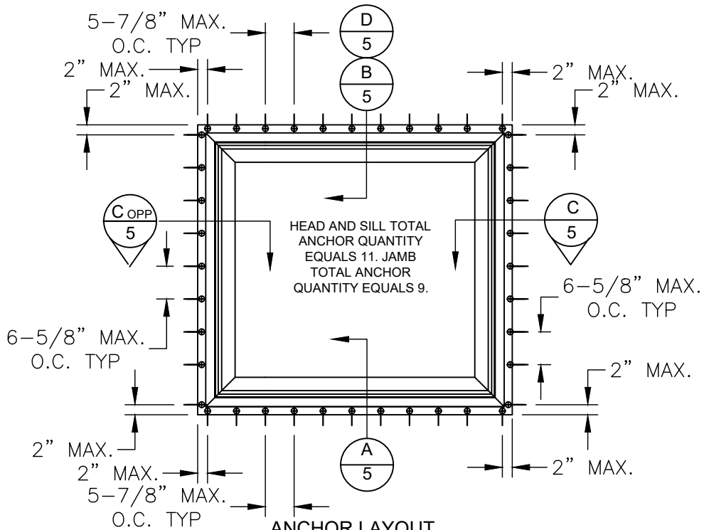
ANCHOR LAYOUT NAILING FIN INSTALLATION
