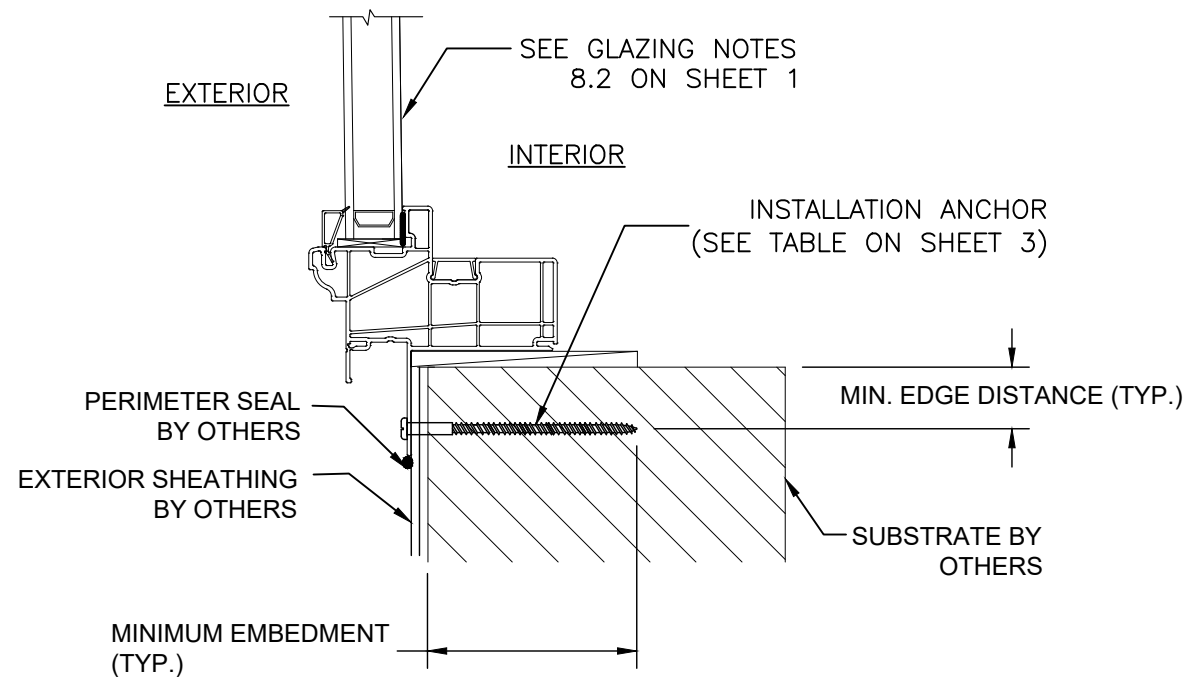
A 5 ANCHOR DETAIL NAILING FIN FRAME SILL
