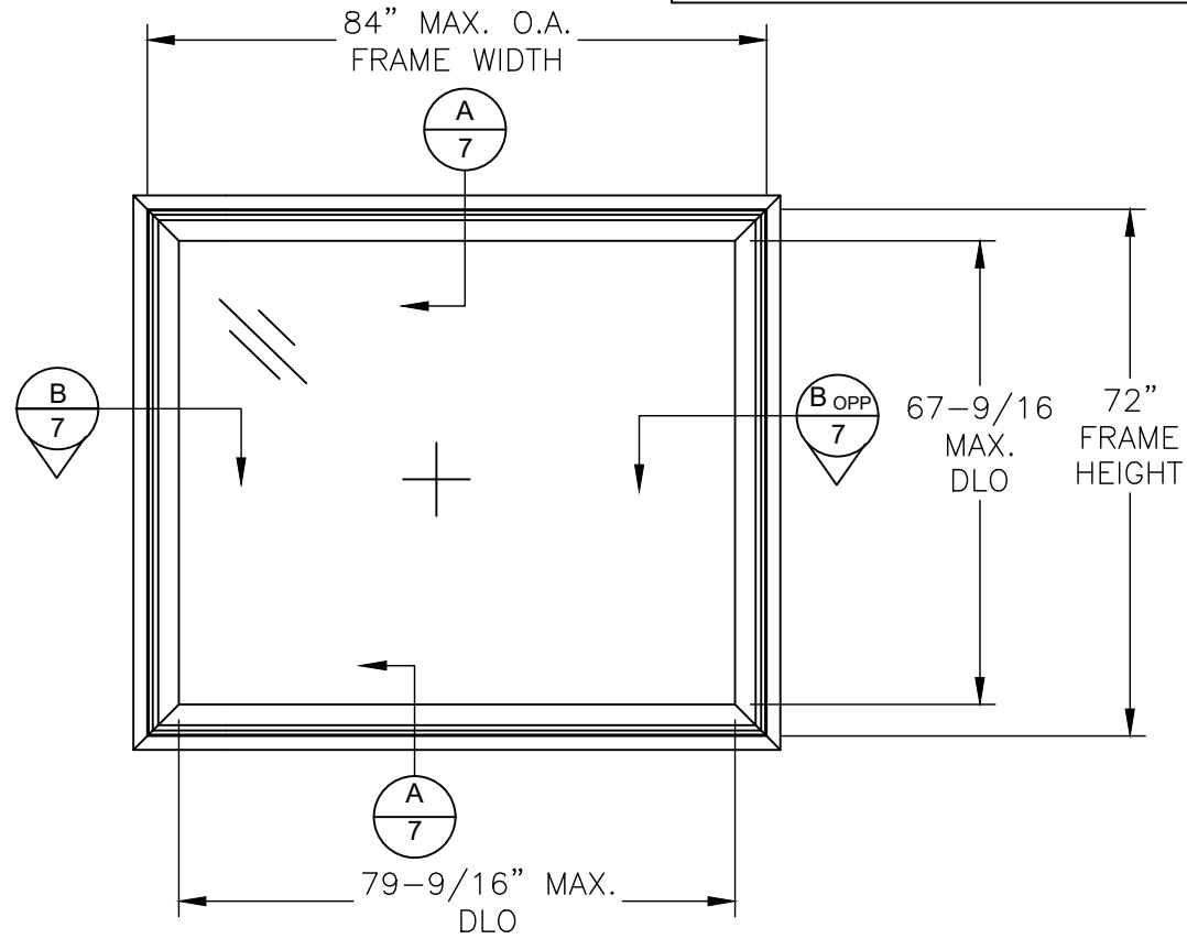
ELEVATION LAYOUT PICTURE WINDOW EQUAL LEG FRAME
