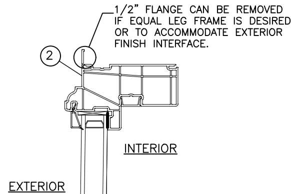
A 8 VERTICAL SECTION FRAME HD/SILL-FLANGED
